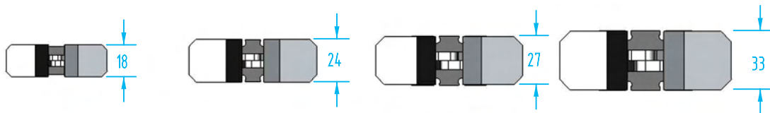
Dimensions with fingers open:
