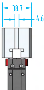
Dimensions with fingers closed: (finger blanks are shown overlapped. Cut away material to fit your part)
