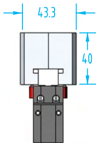
Dimensions with fingers closed: (finger blanks are shown overlapped. Cut away material to fit your part)
