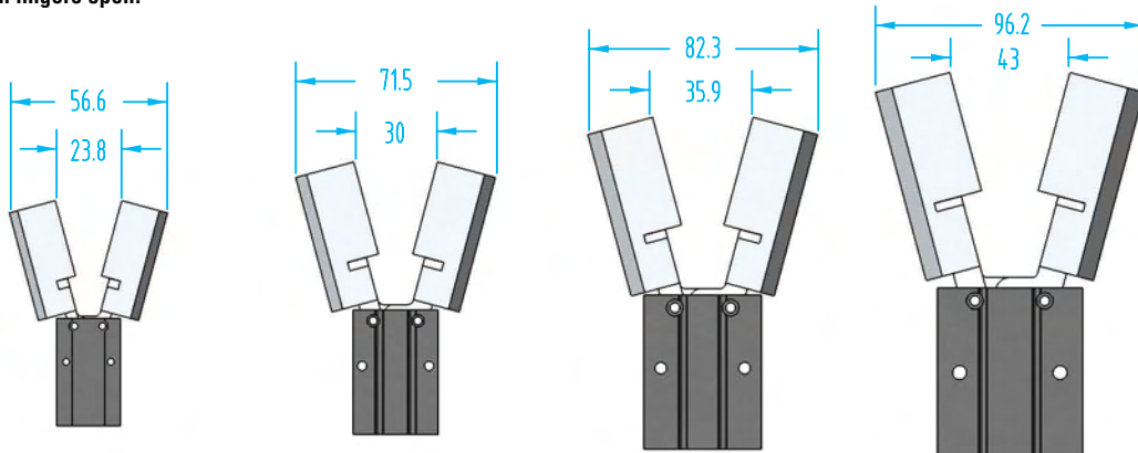
Dimensions with fingers open:
